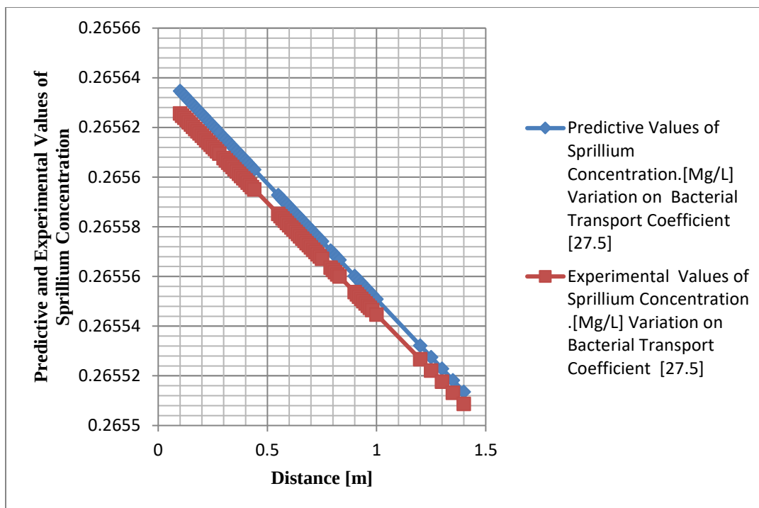
Figure 7: Predictive and Experimental Values of Siplillum Concentration at Different Distance
