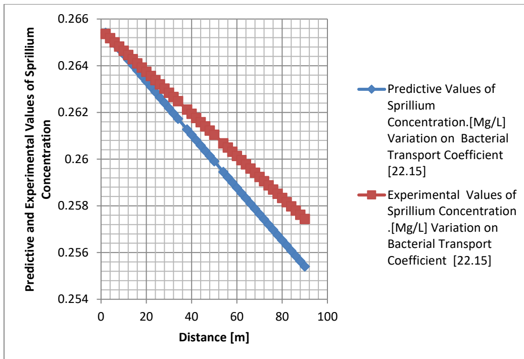
Figure 5: Predictive and Experimental Values of Sipiillum Concentration at Different Distance
