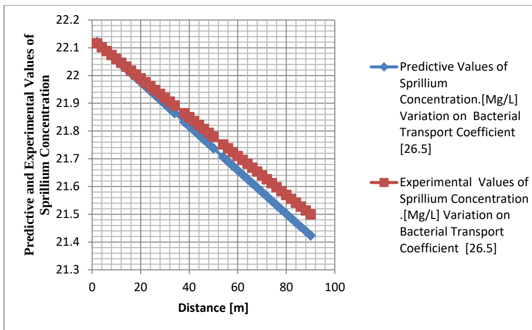
Figure 3: Predictive and Experimental Values of Siproilium Concentration at Different Distance
