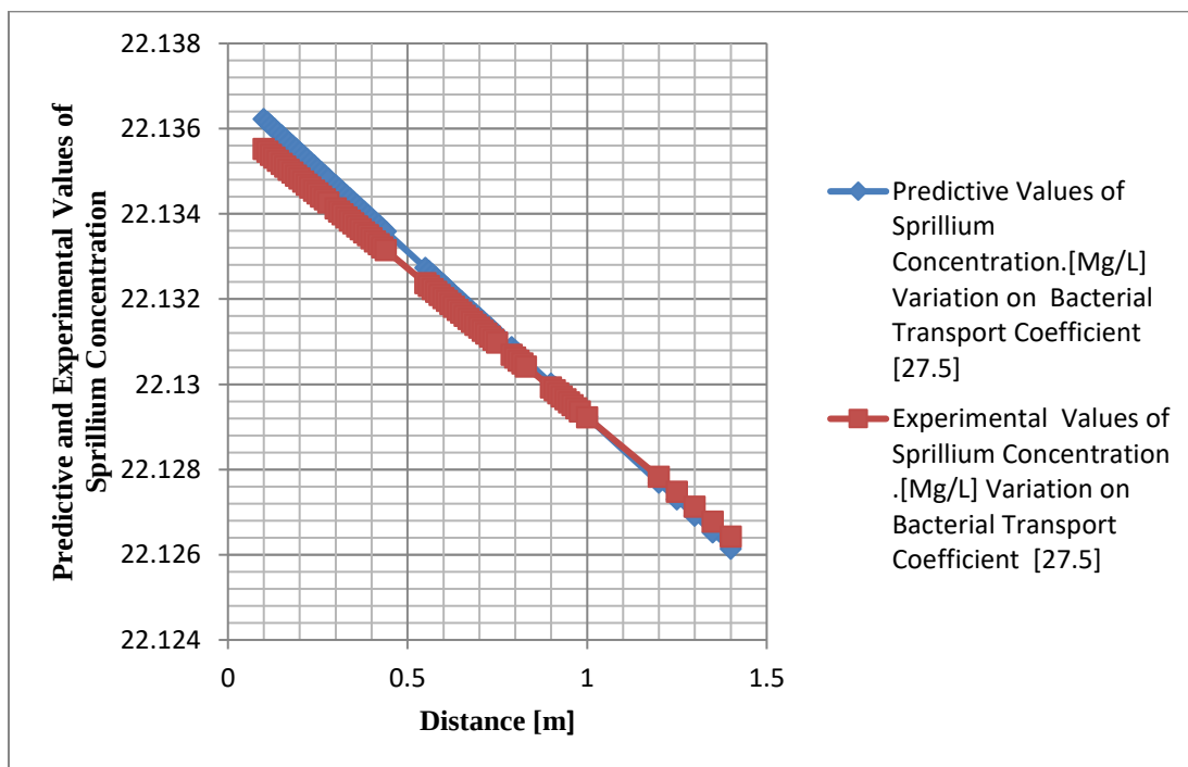
Figure 6: Predictive and Experimental Values of Sipiillum Concentration at Different Distance
