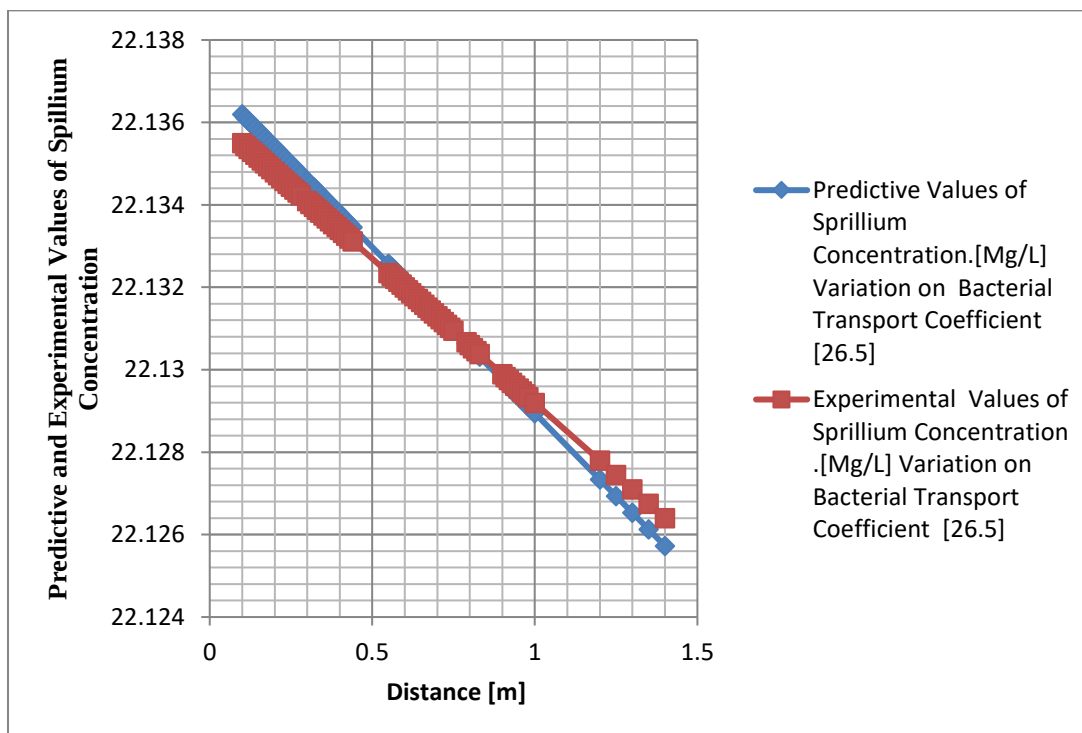
Figure 8: Predictive and Experimental Values of Siplillum Concentration at Different Distance
