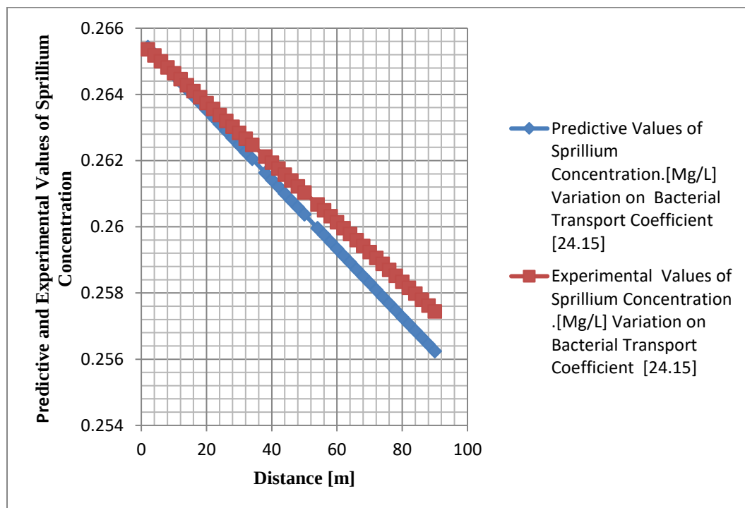
Figure 4: Predictive and Experimental Values of Siproilium Concentration at Different Distance
