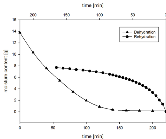
Fig 04: Dehydration-Rehydration curve for 70°C
