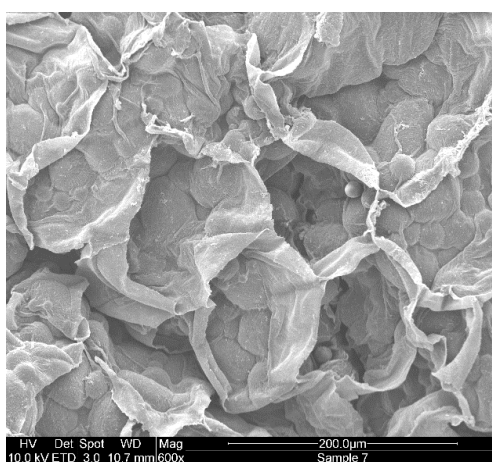
Fig 08: SEM image after drying at 70°C (600 x)
