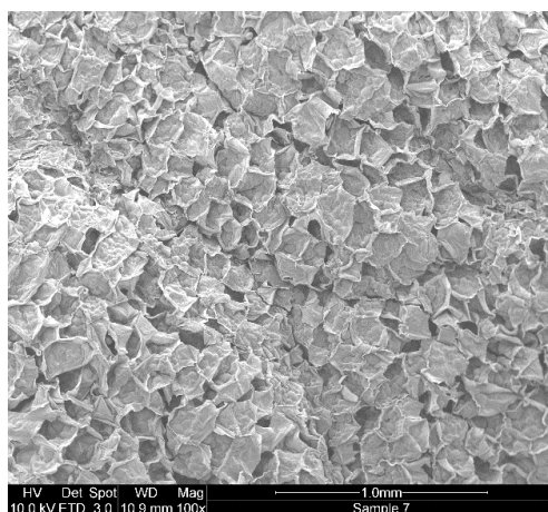
Fig 07: SEM image after drying at 70°C (100 x)
