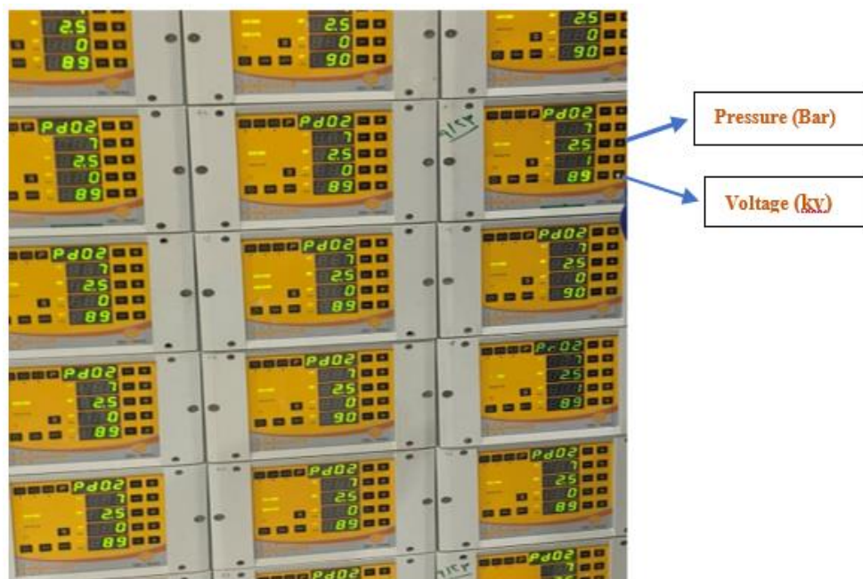
Figure 4: Voltage and pressure setup.
