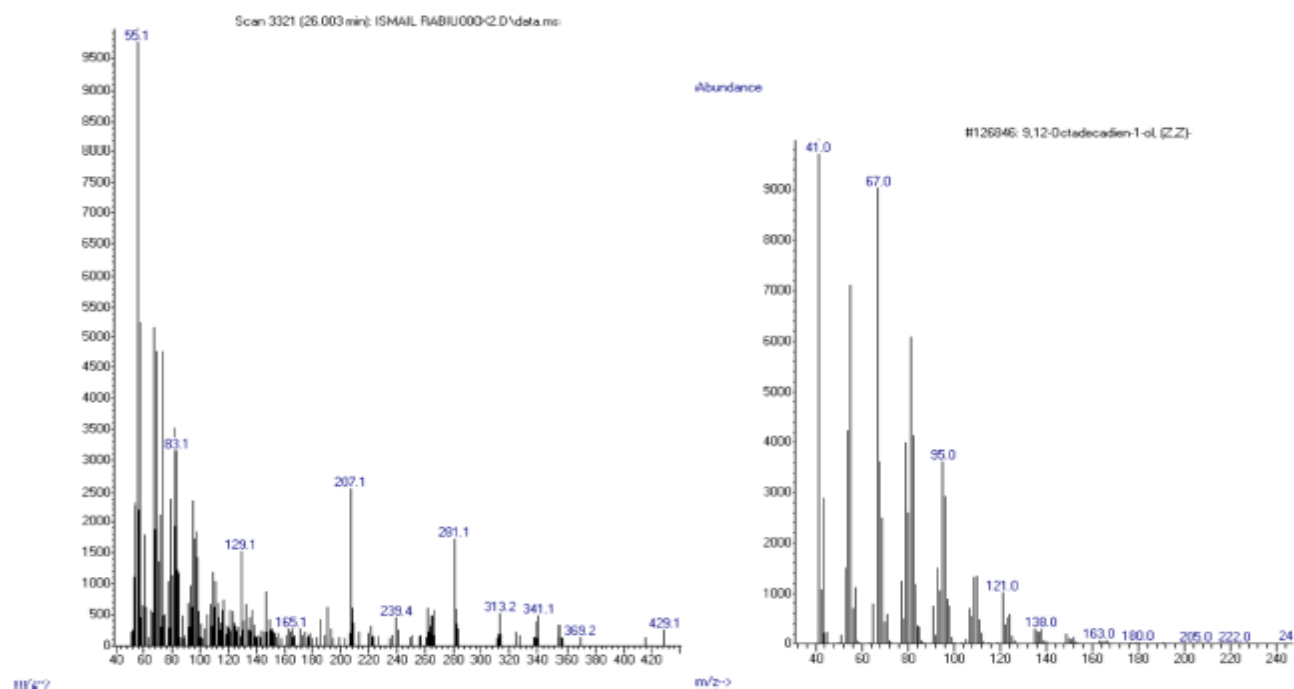
Figure 7 GCMS Chromatogram of the Methanol extracts of C. esculenta showing 9,12-Octadecadienoic acid
