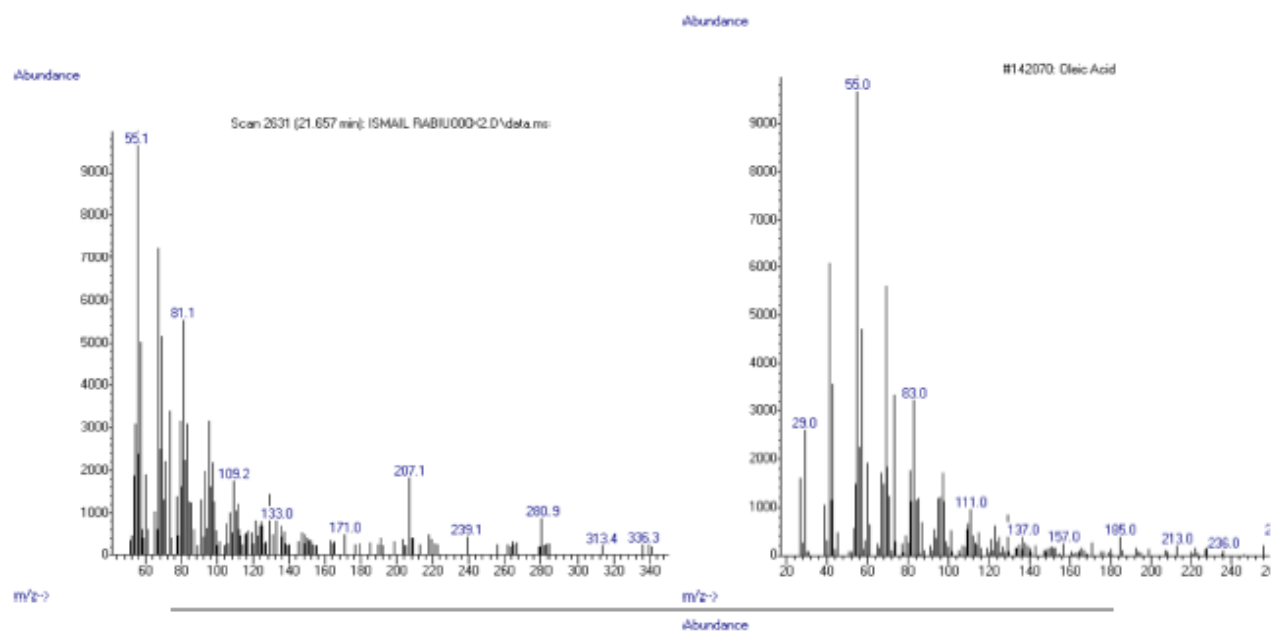
Figure 13 GCMS Chromatogram of the Methanol extracts of M. esculanta showing Oleic Acid
