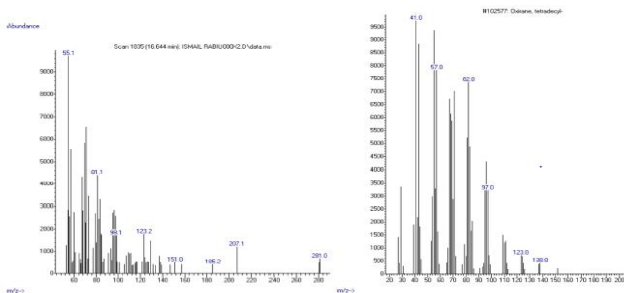
Figure 9 GCMS Chromatogram of the Methanol extracts of C. esculenta showing Oxirane
