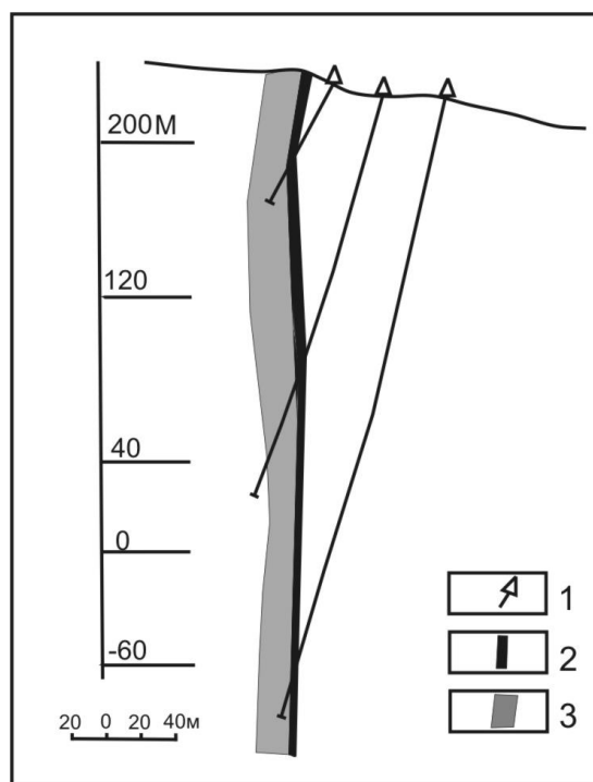
Figure 2 The section of the Poperechnoe's ore body. By (Chebotarev, 1958) the simplification. 1 – Bore holes; 2 – manganese ore stratum at the eastern side of the iron ore body; 3 - Iron ore body.
