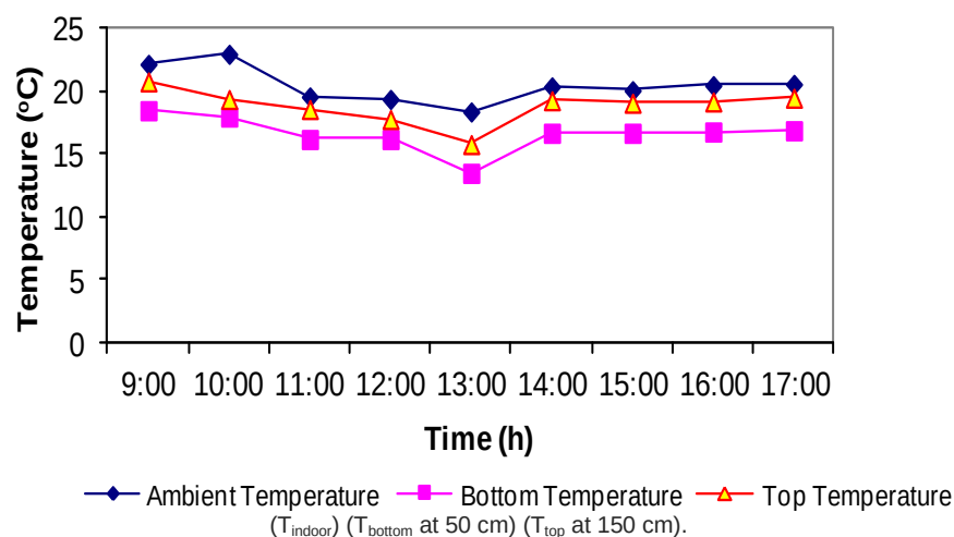
Appendix 2.21. Temperature variation in December.
