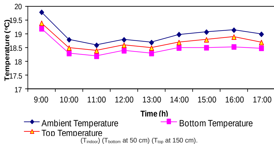
Appendix 2.7. Temperature variation in May.
