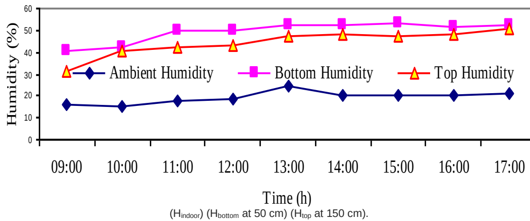
Appendix 2.18. Average daily variation of humidity in October.
