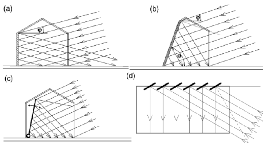
Figure 2 Greenhouse types according to the applied mode of reflection of solar radiation: (a) fixed vertical reflecting wall (b) fixed inclined reflecting wall (c) reflecting wall with variable inclination (d) reflecting wall with louvers
