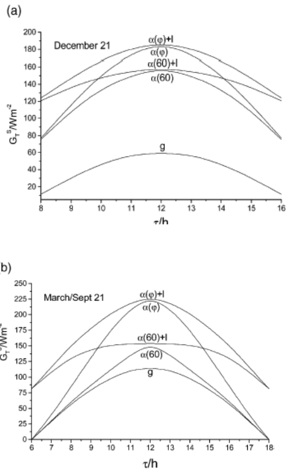
Appendix (1.7). Calculated dependence of ground irradiance on time for the shortest day of the year and for equinox in a greenhouse with a reflecting wall inclined at an angle of 60^\circ , ( \alpha(60) ) with a reflecting wall with variable inclination ( \alpha(\varphi) ), without louvers and ( \alpha(60) + 1 ), ( \alpha(\varphi) + 1 ) the same but with louvers.
