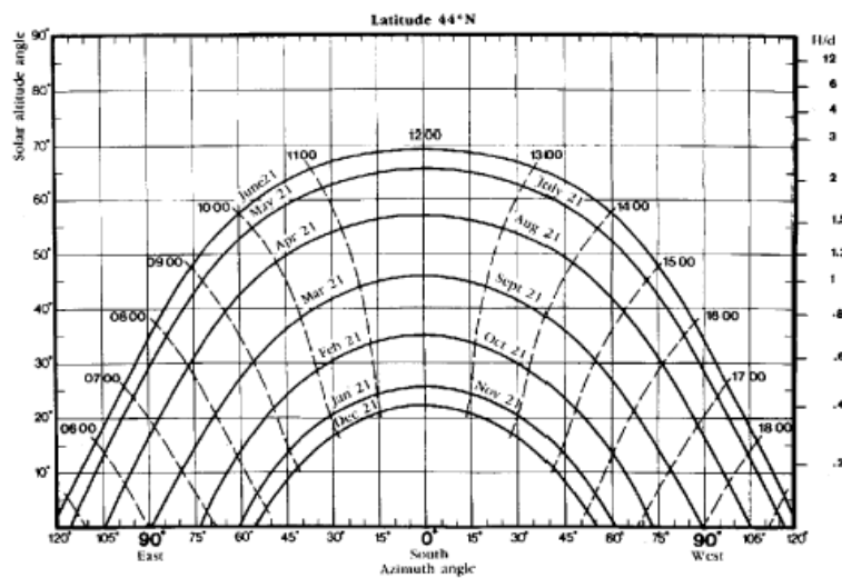
Figure 8 Dependence of the elevation and azimuth angle of the sun on the time of a day at different days of a year at NL 44° [35]
