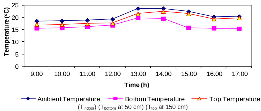
Appendix 2.19. Temperature variation in November.
