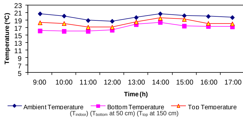
Appendix 2.1. Temperature variation in January.
