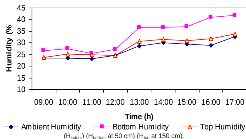
Appendix 5.22. Average daily variation of humidity in December.
