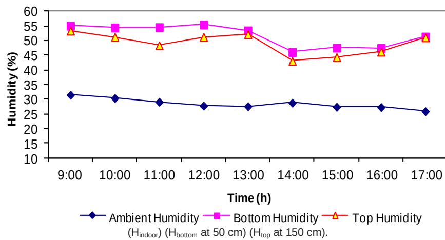
Appendix 2.20. Average daily variation of humidity in November.
