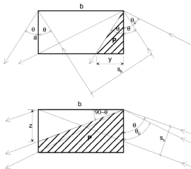
Figure 4 Influence of the azimuth angle \theta \neq 0 on the effectiveness of exposure of the ground to reflected light
