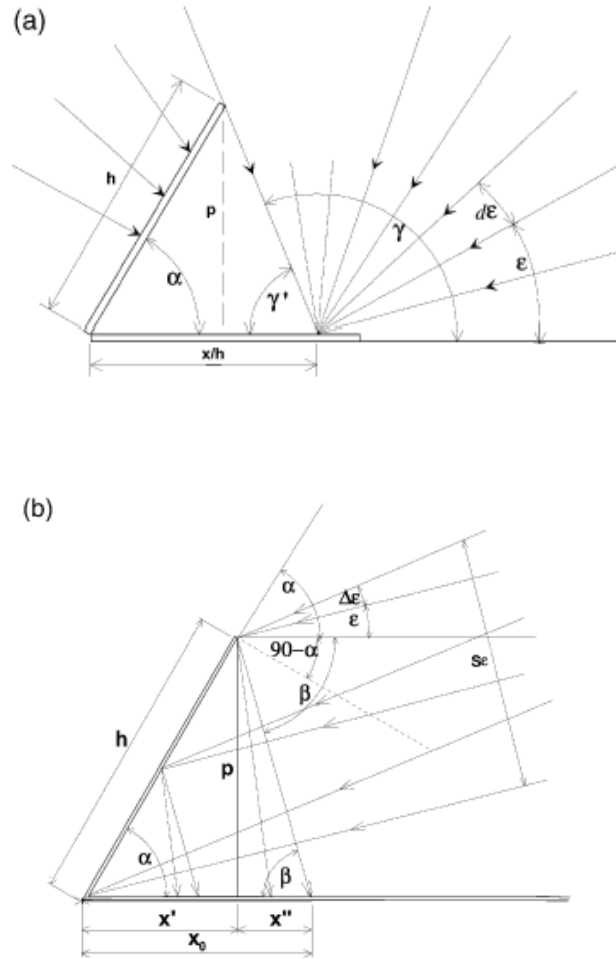
Figure 5 Schematic representations of (a) diffuse light falling onto a point at distance x/h from the reflecting wall, and of (b) diffuse light reflected by the wall.
