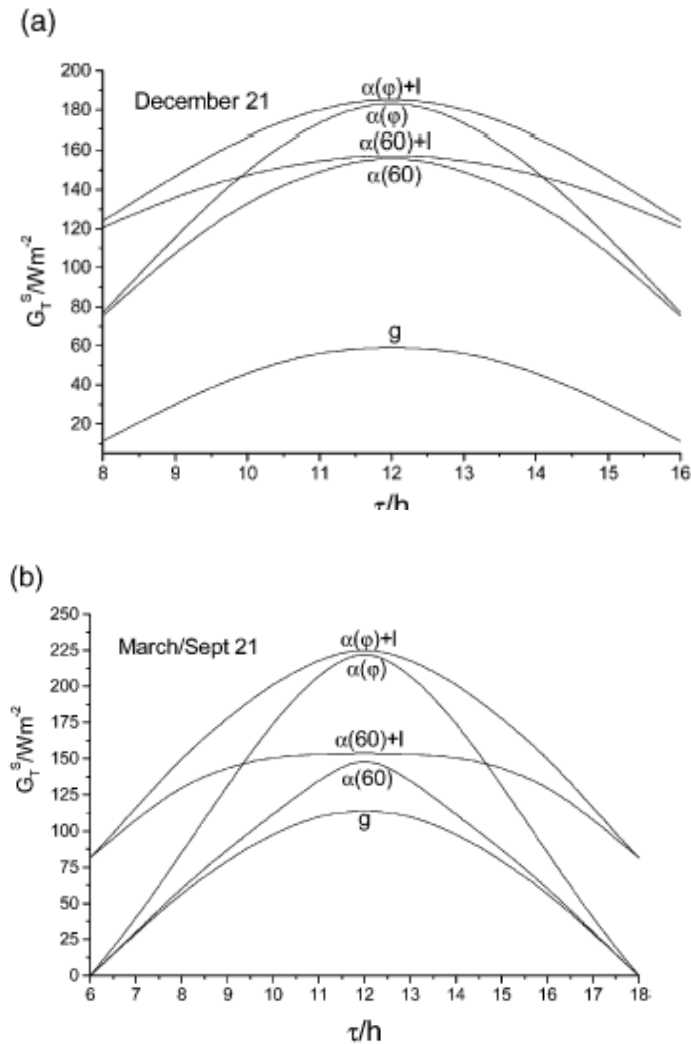
Figure 9 Calculated dependence of ground irradiance on time for the shortest day of the year and for equinox in a greenhouse with a reflecting wall inclined at an angle of 60^\circ , ((\alpha(60))) with a reflecting wall with variable inclination ((\alpha(\varphi)) , without louvers and ((\alpha(60) + 1) , ((\alpha(\varphi) + 1) the same but with louvers
