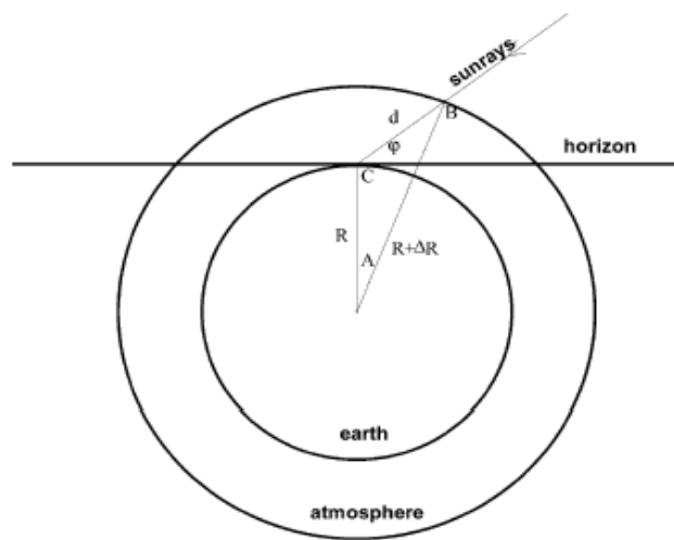
Figure 6 A schematic representations of the earth and its atmosphere with sunrays falling at an inclination \phi with respect to the horizon
