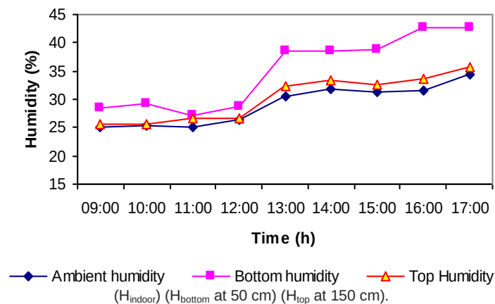
Appendix 2.2. Average daily variation of humidity in January.
