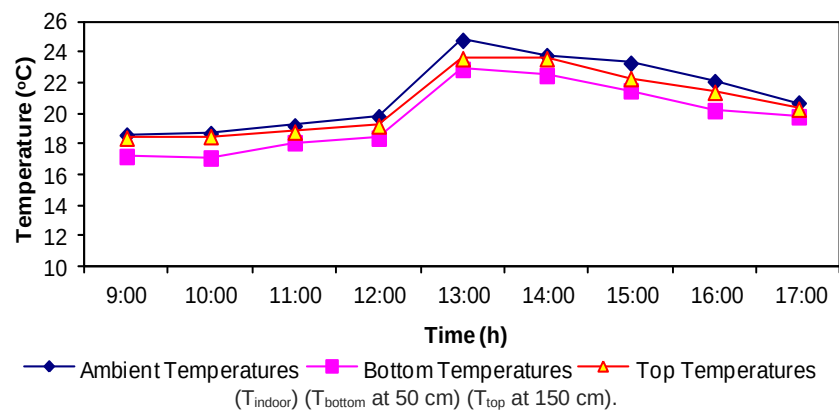
Appendix 2.3. Temperature variation in February.
