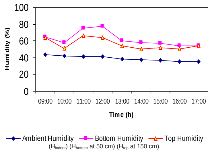
Appendix 2.12. Average daily variation of humidity in July.
